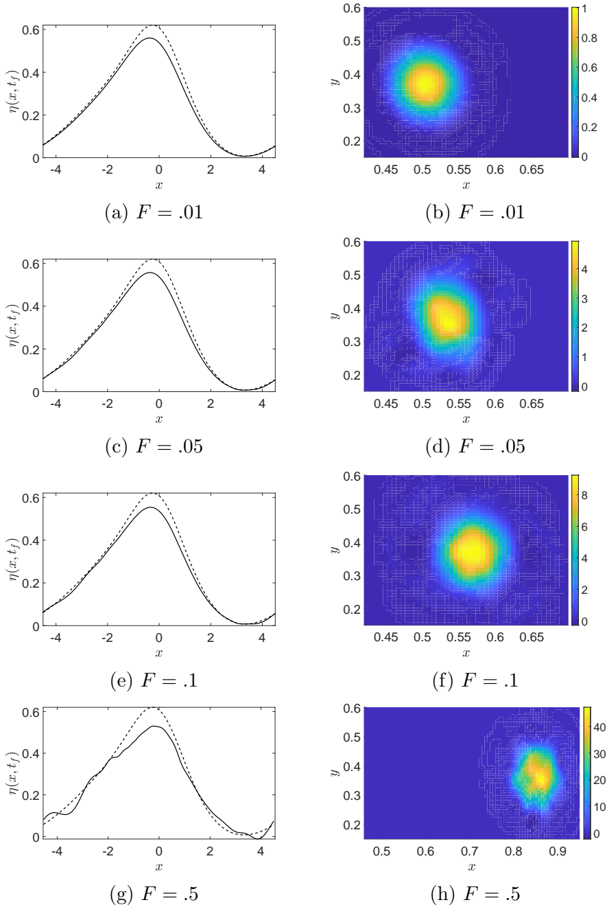
Figure 6: Comparisons of a cnoidal wave over a vortex patch(-) to a cnoidal wave over an irrotational fluid (- -) are shown on the left for various values of the Froude number F , while the final position, shape, and strength of the vortex patch is shown on the right. Here \mu = .2 , \gamma = \sqrt{\mu} , t_f = 2/\mu , \tilde{m} = .6 , \kappa = .43 .
