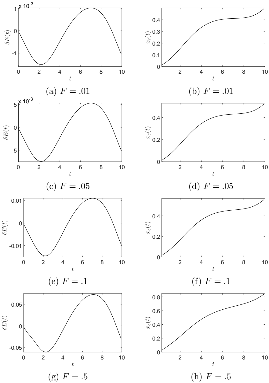
Figure 7: The relative energy input into the free surface is shown on the left, while the motion of the horizontal center of mass x_c(t) is shown on the right for \tilde{m} = .6 and \kappa = .43 .
