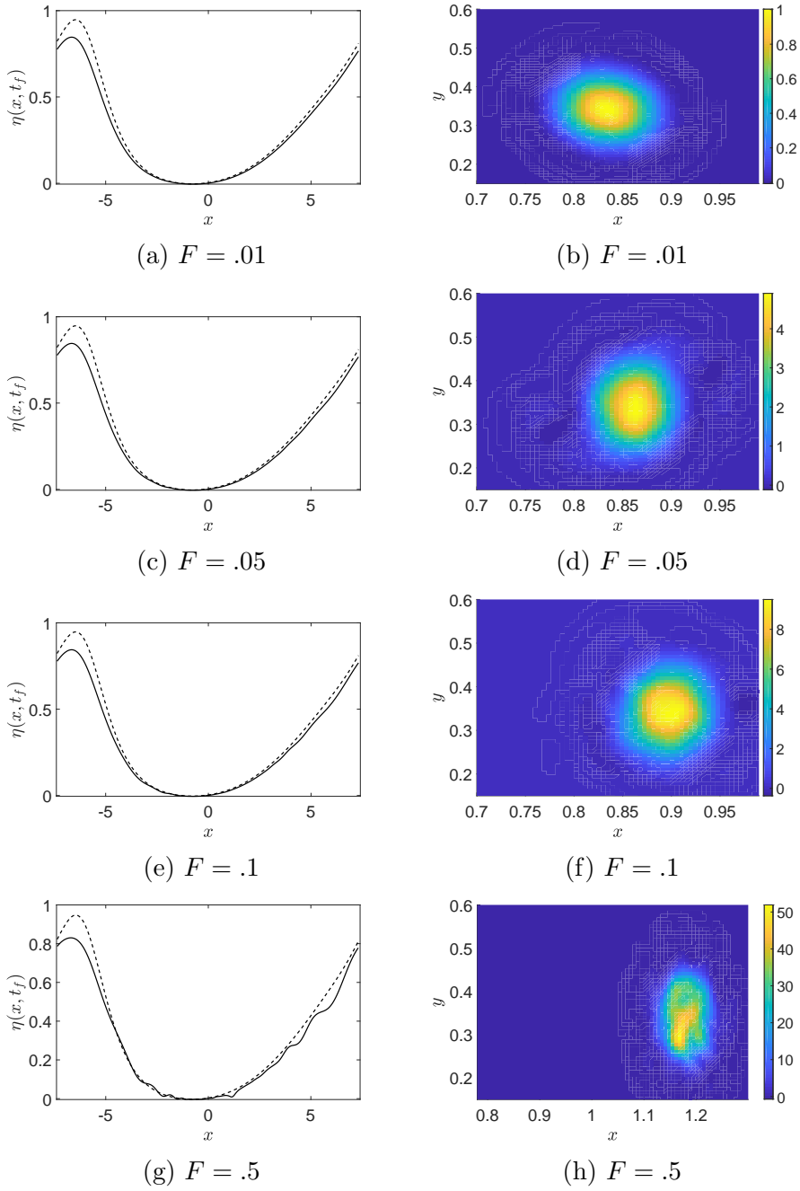
Figure 8: Comparisons of a cnoidal wave over a vortex patch(-) to a cnoidal wave over an irrotational fluid (- -) are shown on the left for various values of the Froude number F , while the final position, shape, and strength of the vortex patch is shown on the right. Here \mu = .2 , \gamma = \sqrt{\mu} , t_f = 2/\mu , \tilde{m} = .9 , \kappa = .35 .
