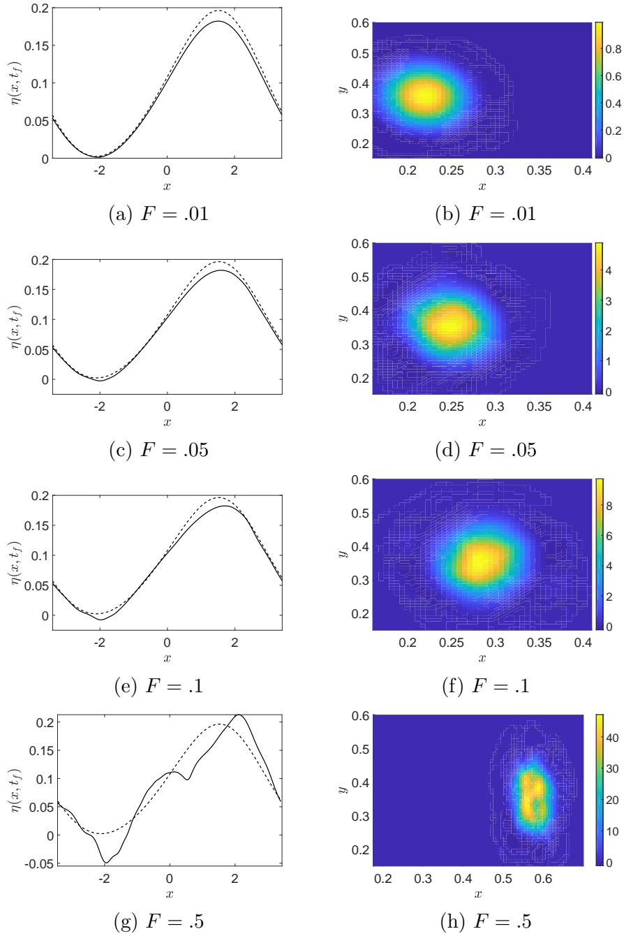
Figure 4: Comparisons of a cnoidal wave over a vortex patch(-) to a cnoidal wave over an irrotational fluid (- -) are shown on the left for various values of the Froude number F , while the final position, shape, and strength of the vortex patch is shown on the right. Here \mu = .2 , \gamma = \sqrt{\mu} , t_f = 2/\mu , \tilde{m} = .3 , \kappa = .5 .
