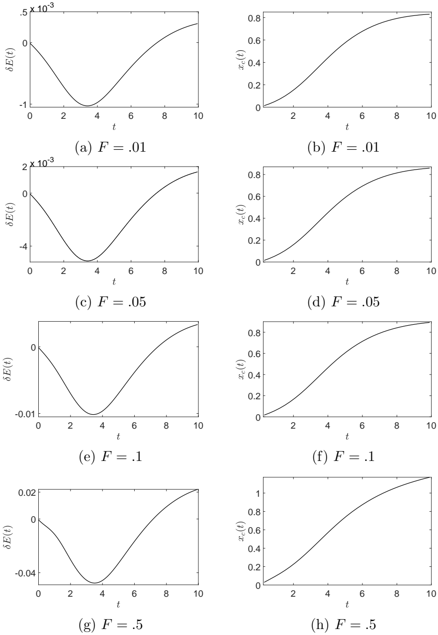
Figure 9: The relative energy input into the free surface is shown on the left, while the motion of the horizontal center of mass x_c(t) is shown on the right for \tilde{m} = .9 and \kappa = .35 .
