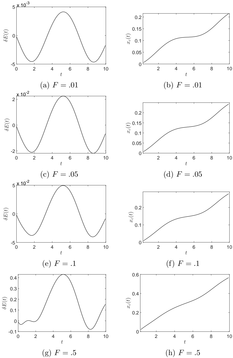
Figure 5: The relative energy input into the free surface is shown on the left, while the motion of the horizontal center of mass x_c(t) is shown on the right for \tilde{m} = .3 and \kappa = .5 .
