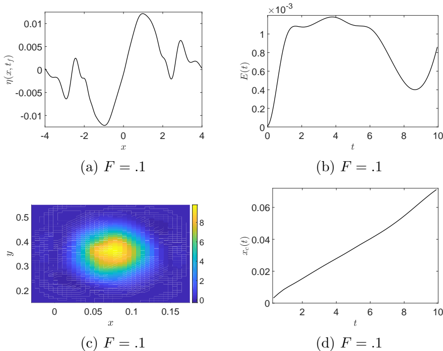
Figure 3: Profile (a), energy input (b), final vortex patch position and shape (c), and motion of the patch's horizontal center-of mass (d) for an initially still surface. Here F = .1 , \mu = .2 , \gamma = \sqrt{\mu} , and t_f = 2/\mu .
