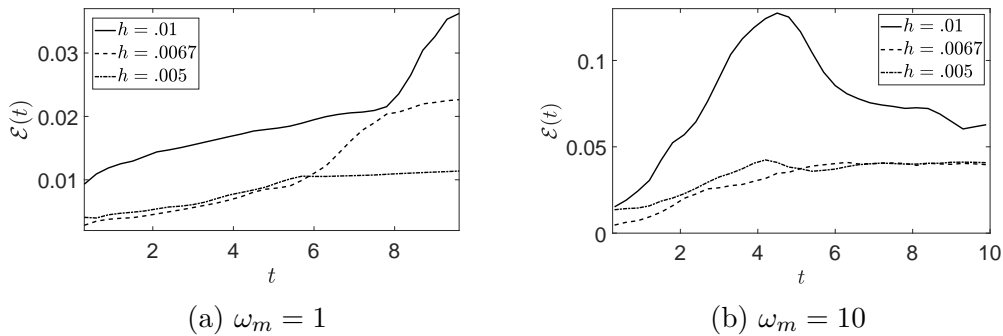
Figure 2: Error profiles for h = .005, .0067, and .01 with \delta = 2h , \omega_m = 1 (a), \omega_m = 10 (b), and regridding done at every six time steps of the simulation.
