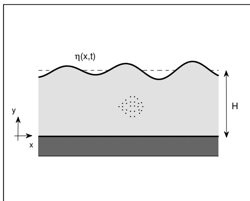
Figure 1: Definition sketch and schematic of a vortex patch approximated by a number of point vortices. In reality hundreds of point vortices are used in the computations.
